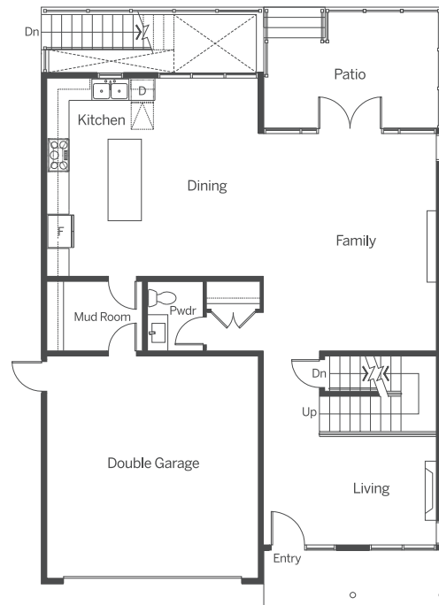
MAIN 1,114 SQ FT
